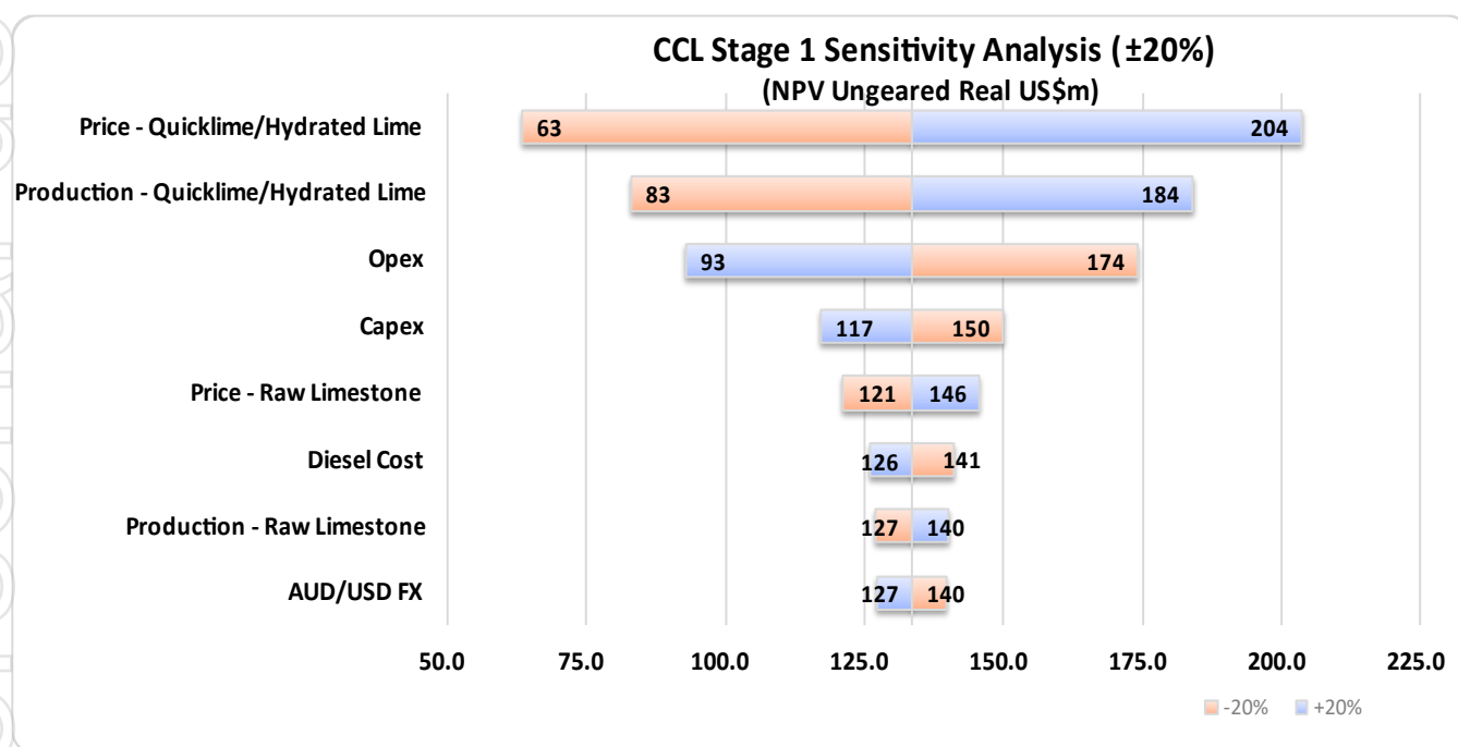
Figure 18 : Sensitivity Analysis
